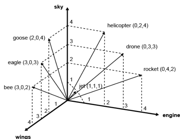
Vector space of seven words in three contexts. 41
